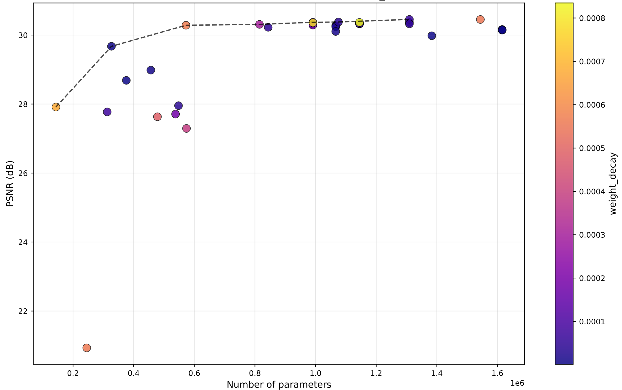
PSNR vs #Params — SRFormer — by weight_decay
